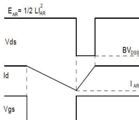
Fig.3-2 Avalanche waveform
