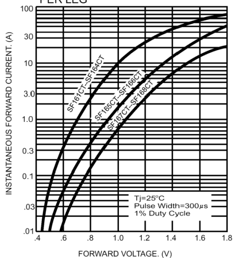
FIG.6- TYPICAL FORWARD CHARACTERISTICS PER LEG
