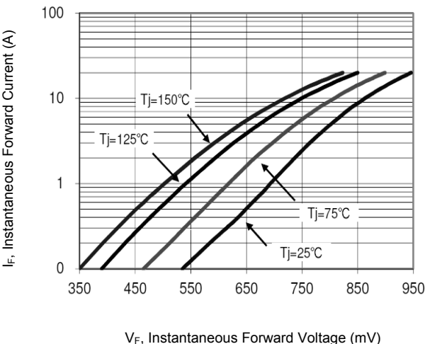
Figure 2. Typical Forward Voltage
