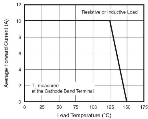
Maximum Forward Current Derating Curve
