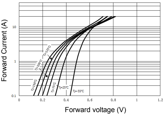
Fig 2. Forward Characteristic Curve
