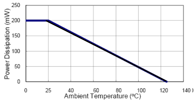
FIG 3 Admissible Power Dissipation Curve
