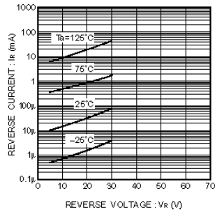
Fig.2 Reverse characteristics
