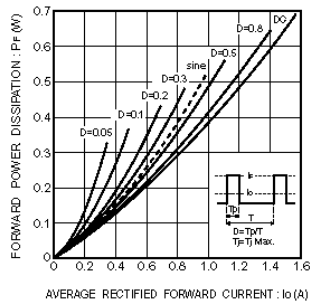
Fig.4 Forward power dissipation characteristics
