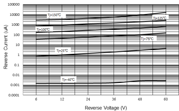
Fig 1. Reverse Current VS Reverse Voltage
