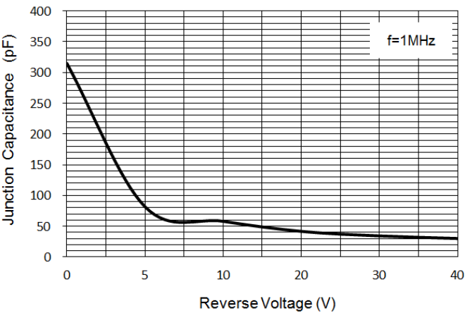
Fig 3. Junction Capacitance
