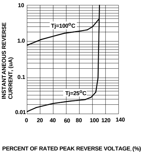
FIG.4-TYPICAL REVERSE CHARACTERISTICS
