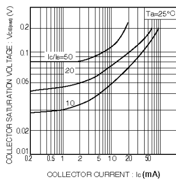
Collector-emitter saturation voltage vs. collector current (I)
