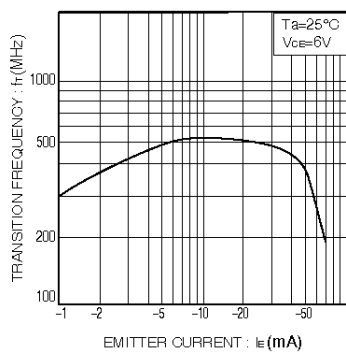
Gain bandwidth product vs. emitter current
