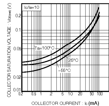
Collector-emitter saturation voltage vs. collector current (II)
