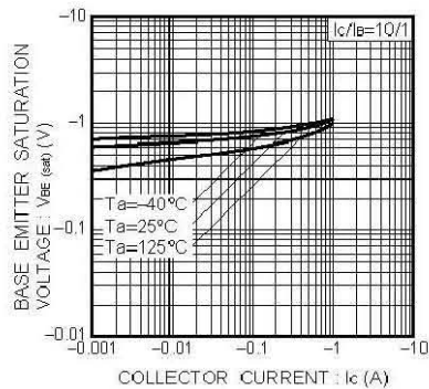
Fig.1 Base-Emitter Saturation Voltage vs. Collector Current
