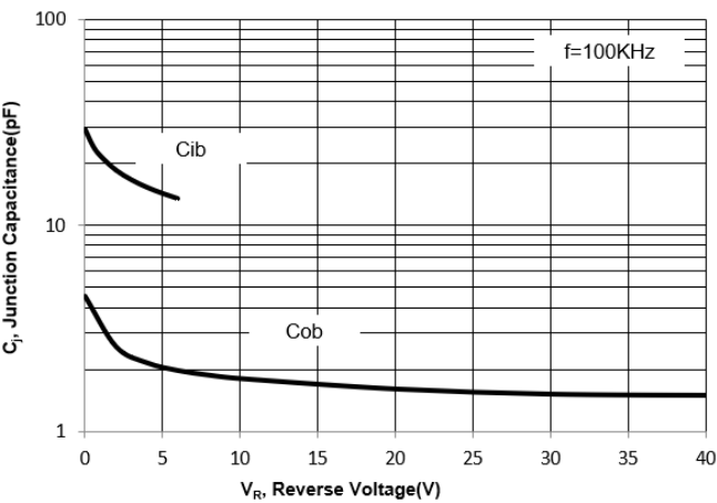
Fig. 7 Junction Capacitance
