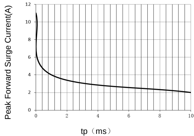
Fig 3. IFSM Curve
