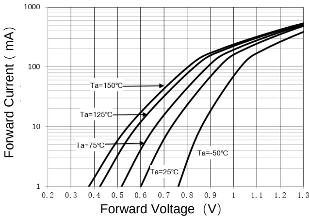
Fig 2. V_F characteristics
