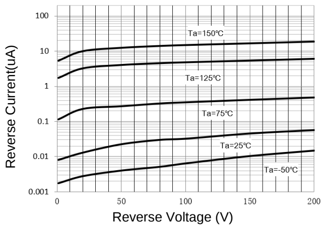
Fig 1. V_R characteristics
