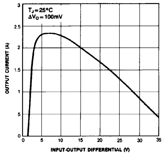
Figure 2. Peak Output Current
