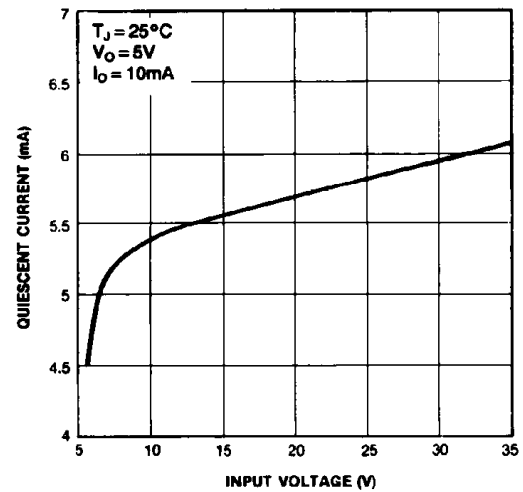
Figure 4. Quiescent Current
