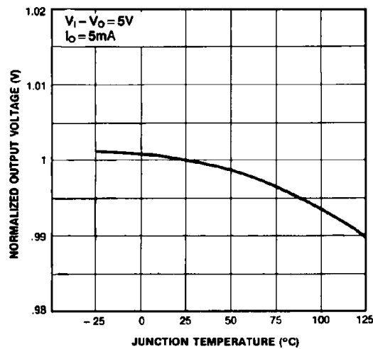
Figure 3. Output Voltage
