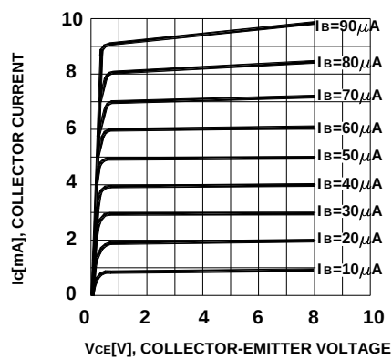
Figure 1. Static Characteristic
