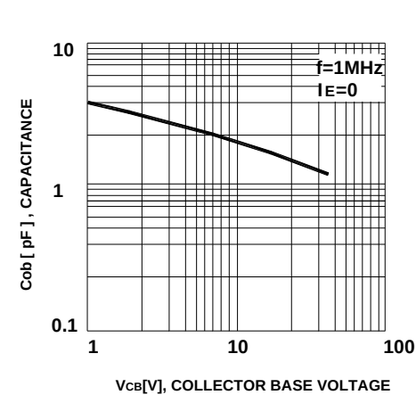
Figure 5. Collector Output Capacitance
