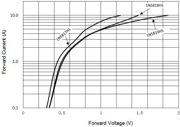
Fig 3. Forward Characteristics
