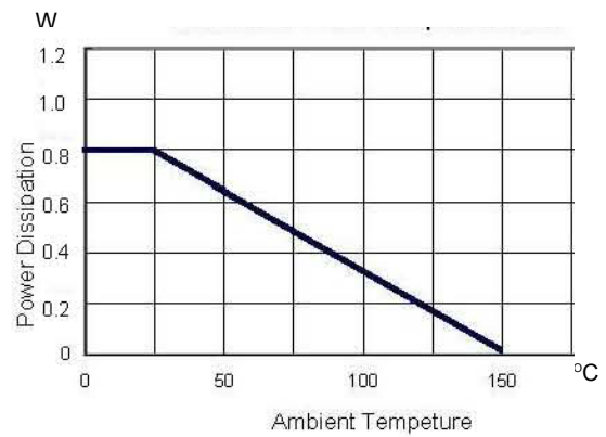
Figure 6. Power Derating
